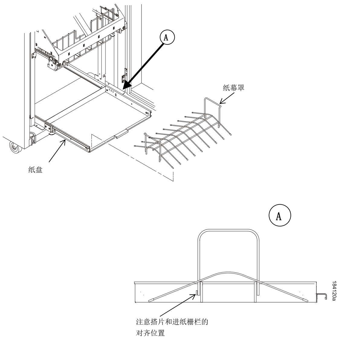
图29. 纸幕罩
